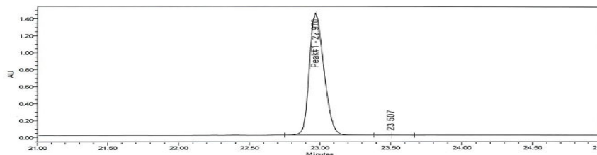
HPLC-UV Chromatogram
